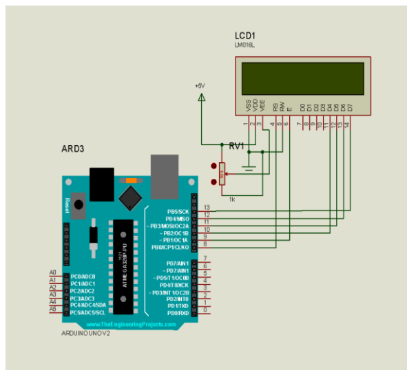
Fig. 1: Connection of the Arduino Uno to Liquid Crystal Display (LCD)
