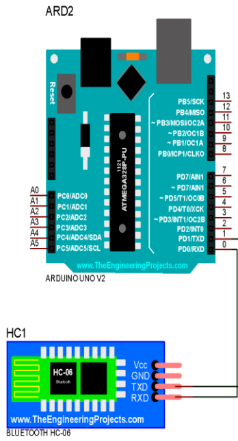
Fig. 3: Connection of the Arduino Uno to the Bluetooth Module
