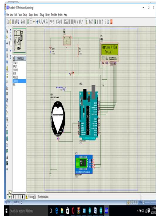
Fig. 7: Result displaying the complete setup of the simulation and the research title
