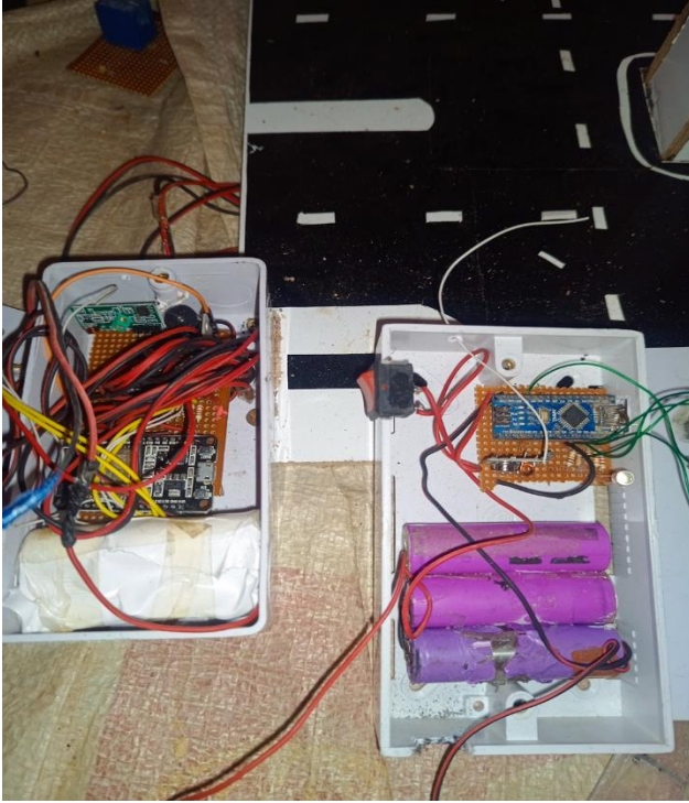
Figure 3: The internal circuitry of the two controllers
