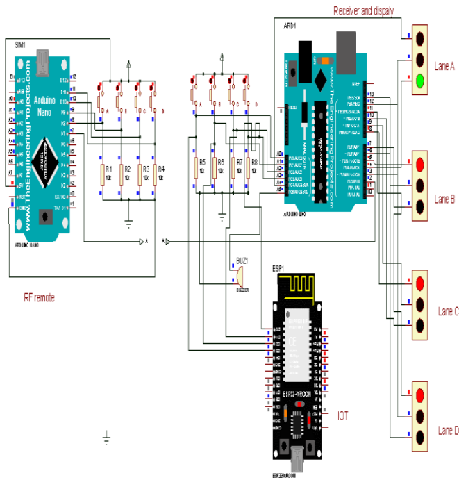
Figure 1: Configuration of the whole simulation system
