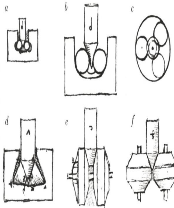
Figure 1: Historical sketches of ball, roller, and taper bearings devised by Leonardo da Vinci
